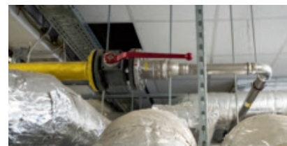
Natural gas pipeline with renewed, tapered piping on the right
