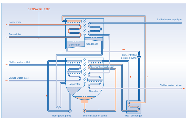
Simplified process scheme of absorption chiller with OPTISWIRL 4200
