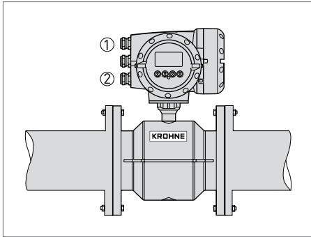
Fig. 48: EMF in compact version (KROHNE, OPTIFLUX 4300C) ① Power supply ② Output signal e.g. 4–20 mA
