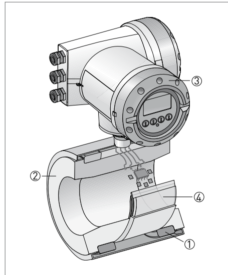
Fig. 26: Structure of an EMF with capacitive signal pick-up ① Field coils ② Measuring tube ③ Signal converter ④ Capacitive electrodes
