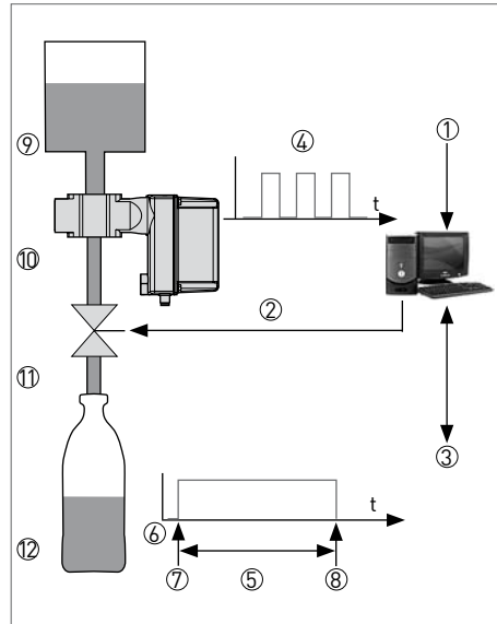
Fig. 37: Volumetric filling with KROHNE BATCHFLUX EMF
