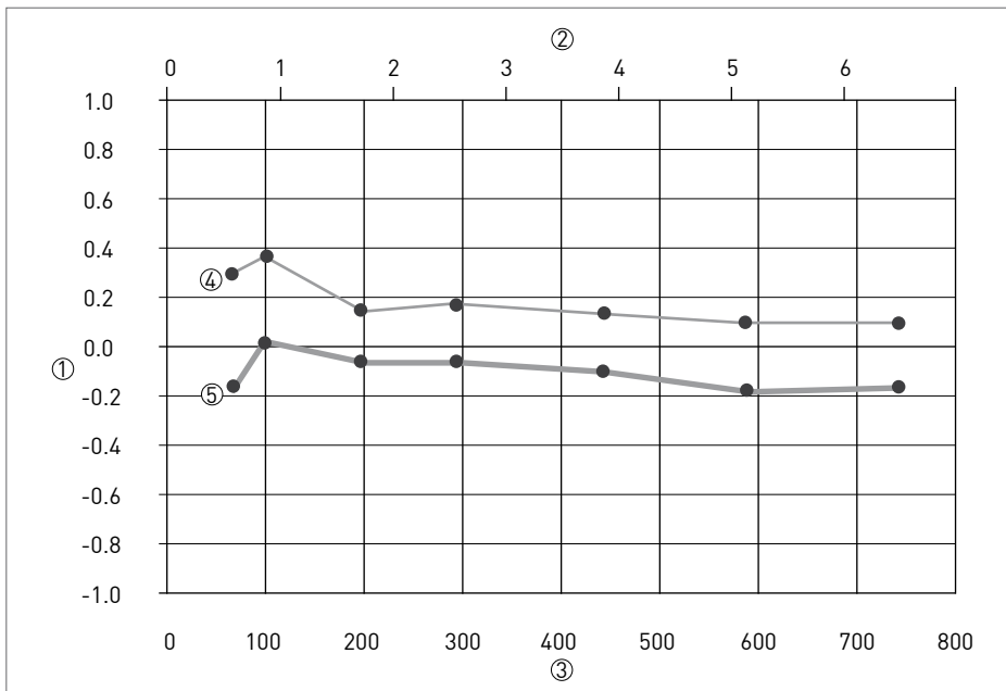
Fig. 14: Effect of the flow profile on EMF measuring accuracy, here using a WIB-SIREP-E-1747-S-94 test with a KROHNE EMF with a nominal size of DN 50 ① Measuring error (% of measured value)
