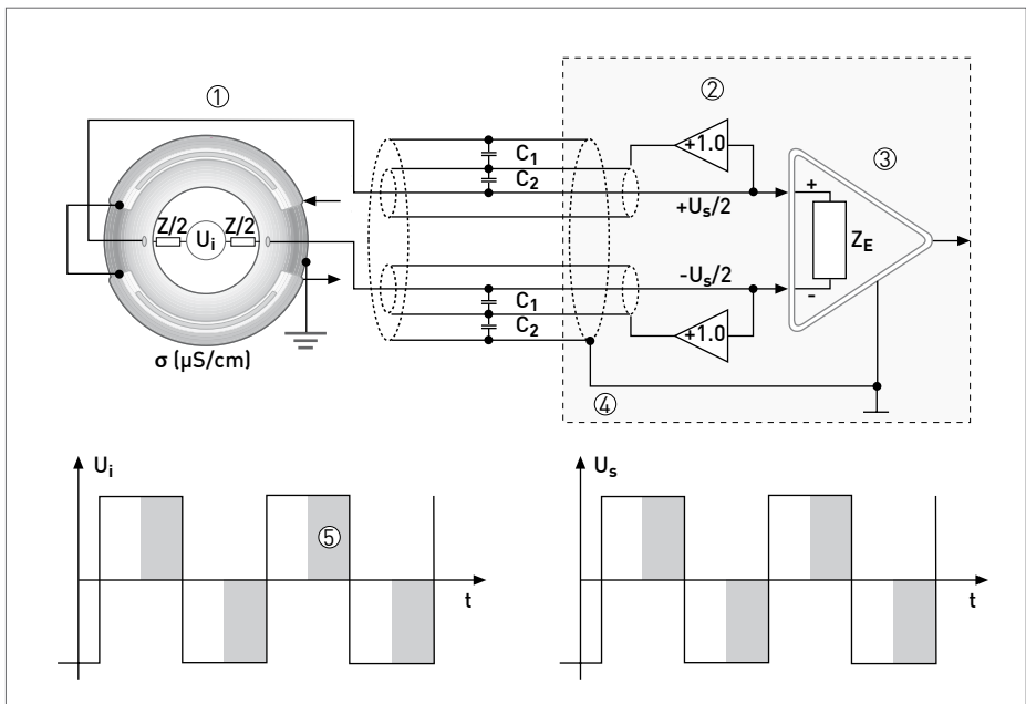
Fig. 64: Line capacitance and signal distortion for signal cable with shielding (Bootstrap) ① Primary head ② Impedance converter
