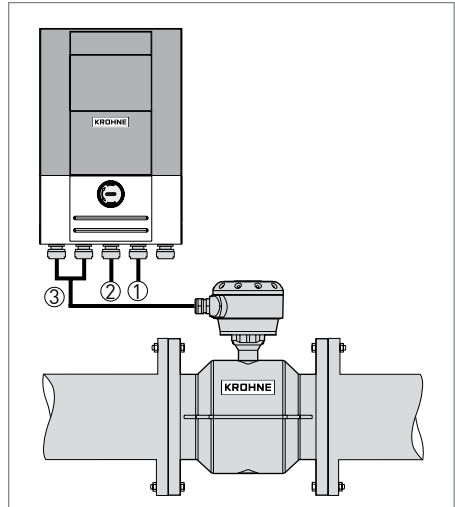
Fig. 49: EMF – remote version (KROHNE, OPTIFLUX 4300W) ① Output signal e.g. 4–20 mA ② Power supply ③ Field current + electrode signal
