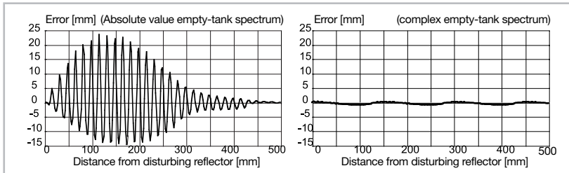
Fig. 45: Measuring errors caused by an interfering reflector: evaluation with the absolute-value empty- tank spectrum (left) and complex empty- tank spectrum (right)
