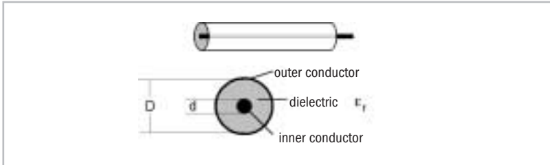
Fig. 12: Coaxial cable
