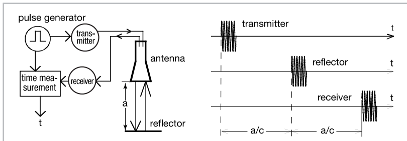
Fig. 5: Pulse radar measuring system
