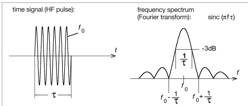
Fig. 6: Time signal and spectrum of a radar pulse
