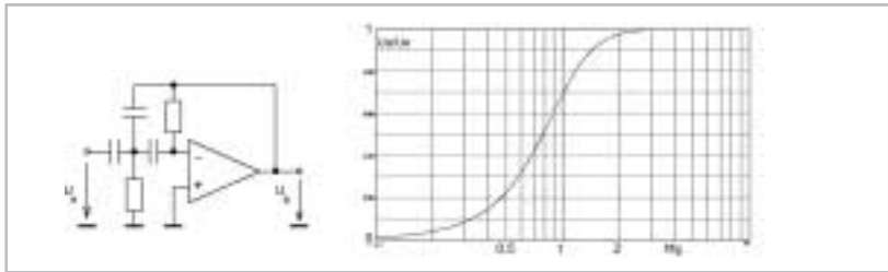
Fig. 41: A high-pass filter and its filtering characteristics
