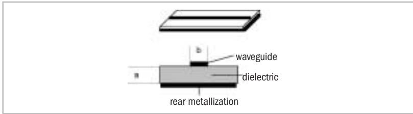
Fig. 14: Planar line
