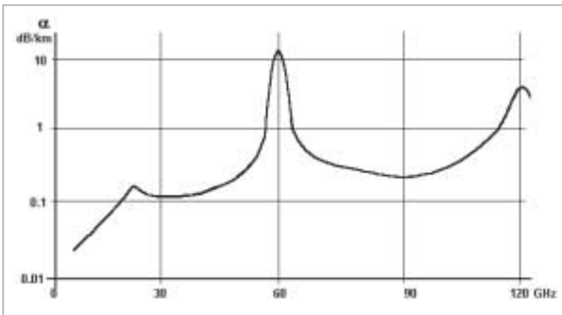
Fig. 26: Attenuation of microwaves in air.
