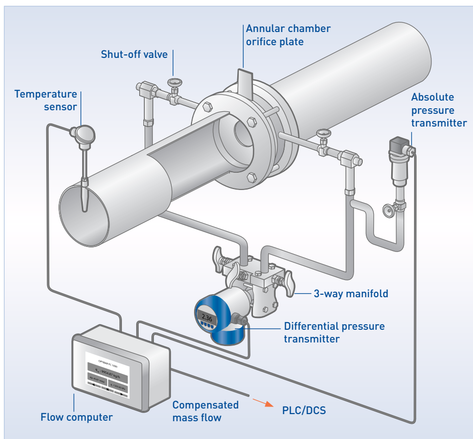
Complete DP flow measuring point for compensated volume/mass flow
