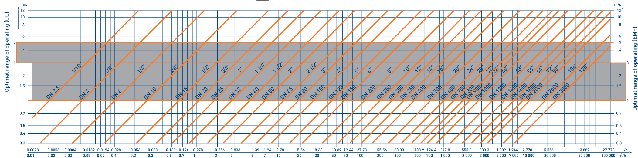
Sizing graph for measurement of liquids | Electromagnetic flowmeters (EMF) | Ultrasonic flowmeters (UL)
