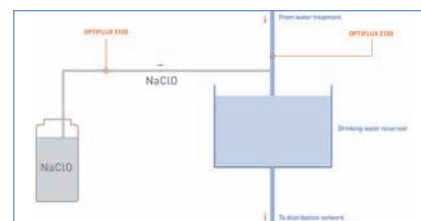
Simplified process flowsheet with measurement points of OPTIFLUX 5100 and OPTIFLUX 2100
